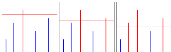
Figure 1: Sequential linearizations in computing hierarchical word error rate. The heights of the vertical lines represent the prominences of boundaries, and each horizontal line is one linearization. In the first step, only the highest boundary is used, producing just two segments. Each following step includes one more boundary.
